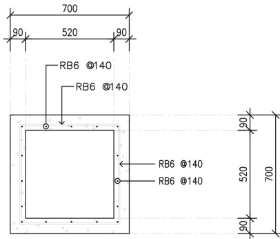
PLAN DETAIL MANHOLE - 40
